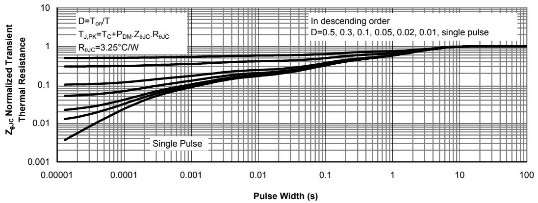
Figure 13: Normalized Maximum Transient Thermal Impedance for AOTF7N60 (Note F)
